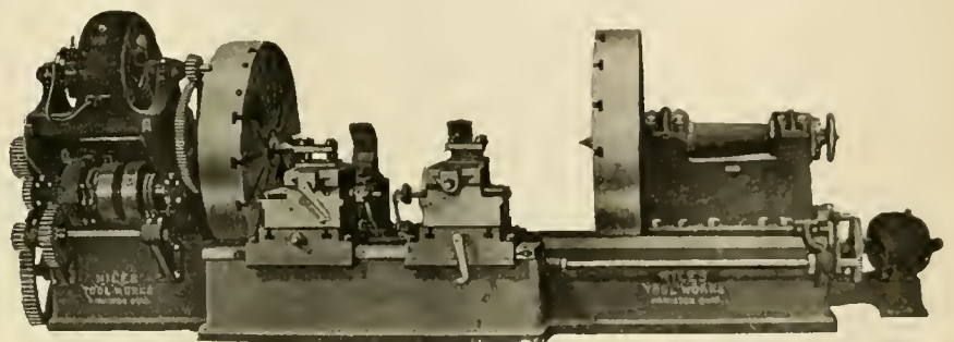
EXTRA HEAVY DRIVING WHEEL LATHE—NILES WORKS.
